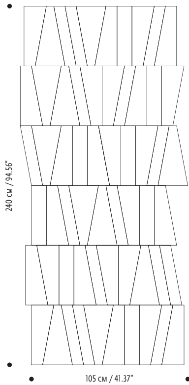
posa 1 / layout 1
