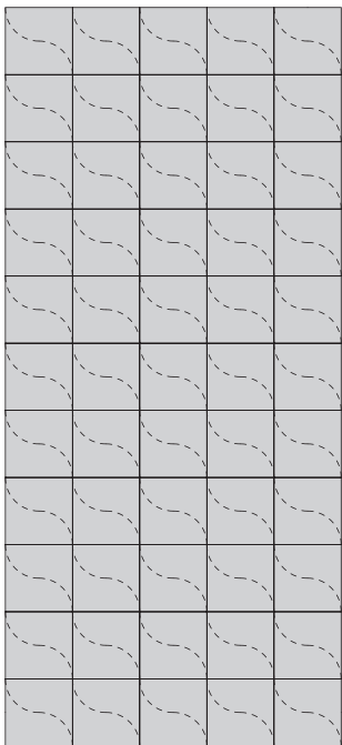
posa 4 / layout 4
